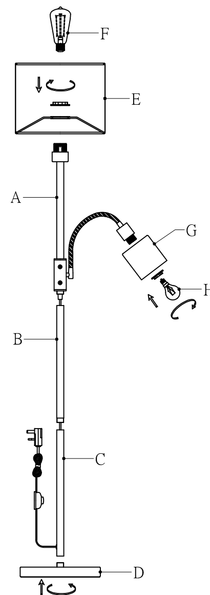
DIAGRAM 2: LAMP ASSEMBLY
