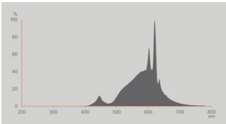
Spectral diagram 1906 SFIL
