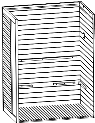
4 Right board
