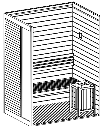
9 Sauna stove
