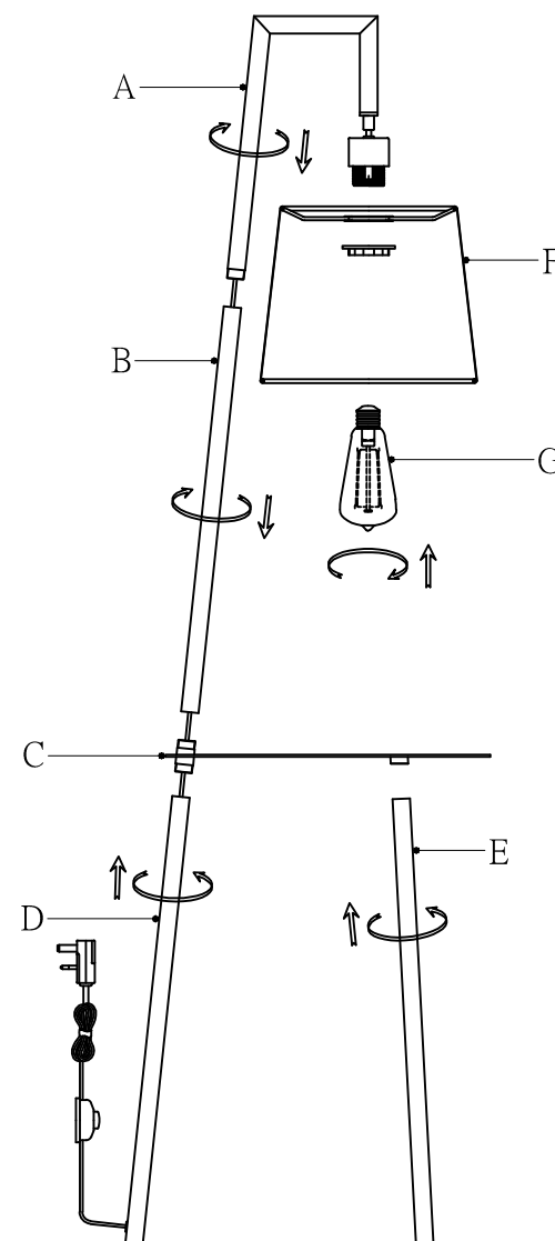
DIAGRAM 2: LAMP ASSEMBLY
