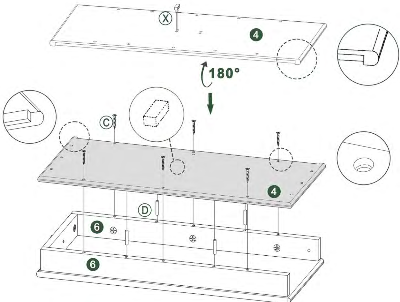
Assembly - B
