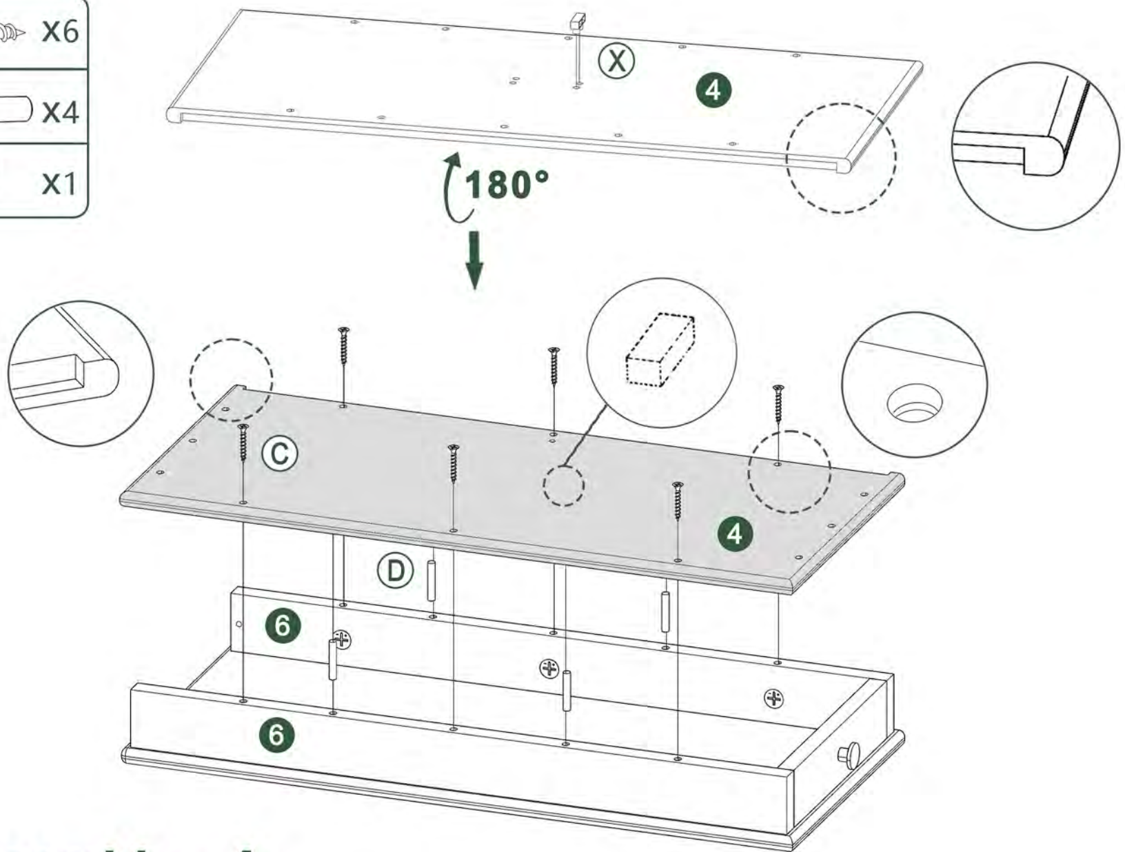
Assembly - A
