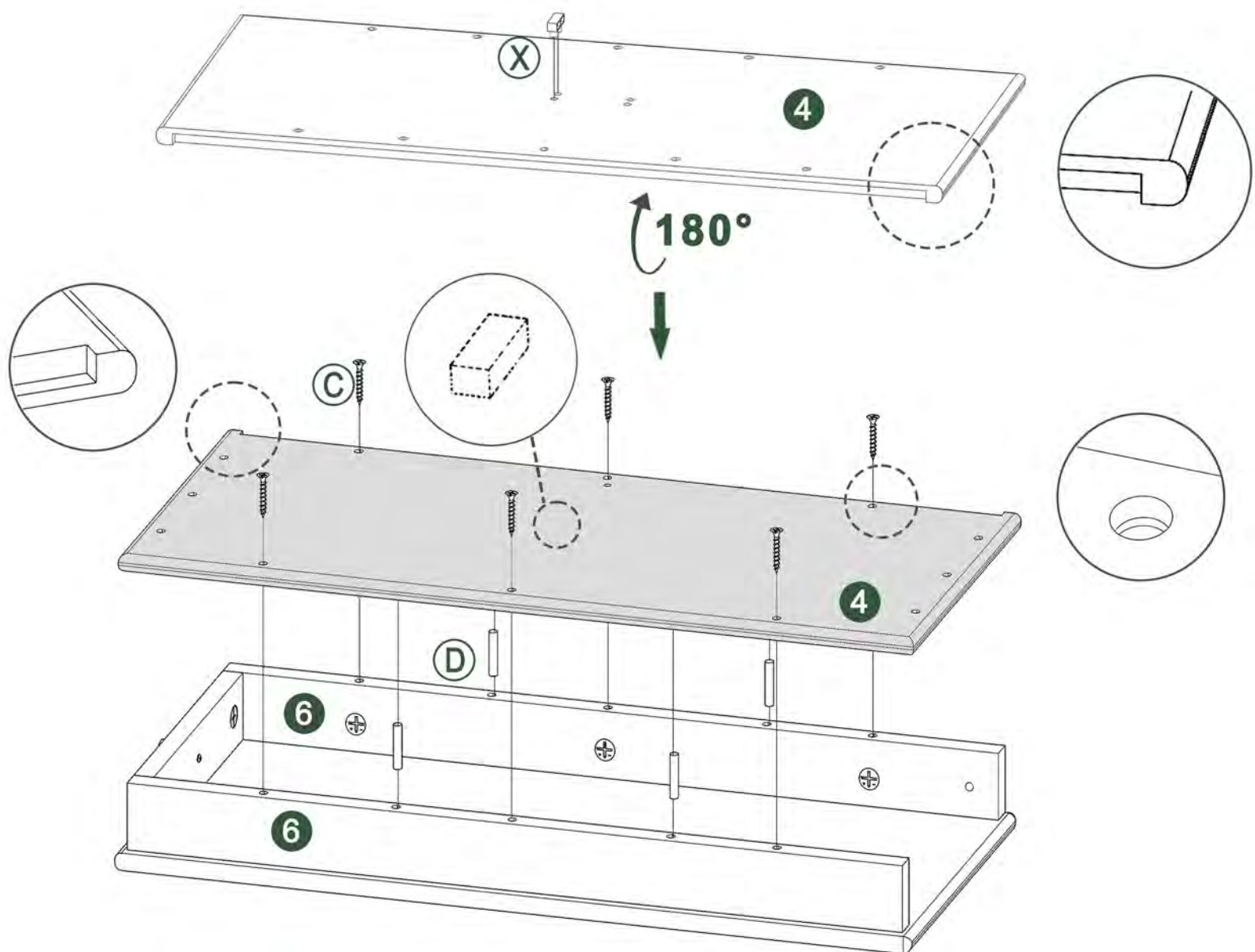
Assembly - B
