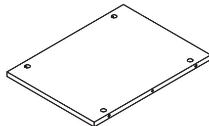
8 Back Panel (430 x 322 x 15mm)
