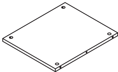
9 Shelf Board (382 x 322 x 15mm) (x2)
