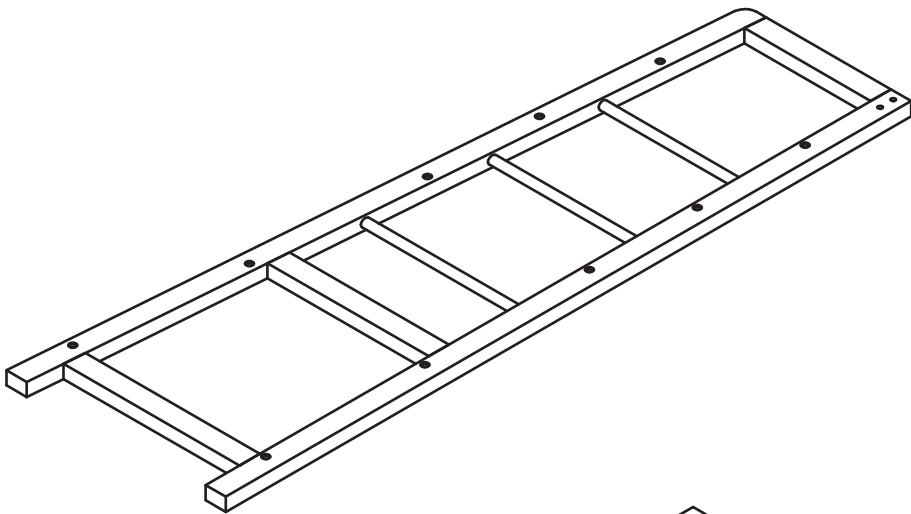
1 Left Frame (1250 x 400 x 24mm)
