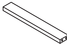
11 Support Rail (352 x 50 x 19mm)
