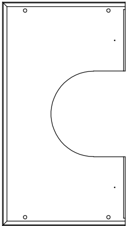
1 Top panel (600 x 330mm)
