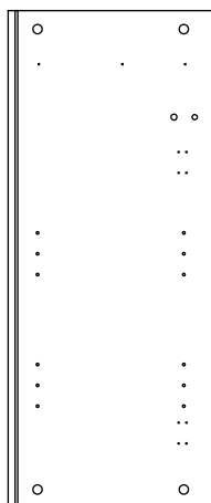
2 Right side panel (760 x 315mm)
