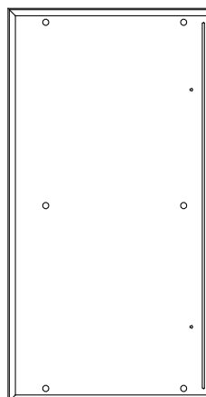
3 Top panel (640 x 330mm)
