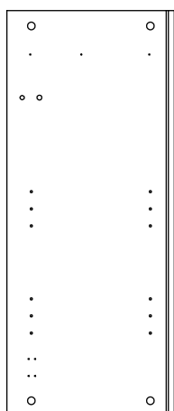
1 Left side panel (760 x 315mm)
