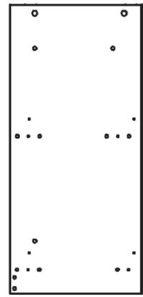
6 Left Panel (Cabinet) (824 x 396 x 15mm) x1
