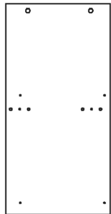
8 Center Support Panel (Cabinet) (748 x 373 x 15mm) x1
