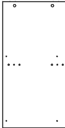
4 Center Support Panel (Cabinet) (748 x 373 x 15mm) x1
