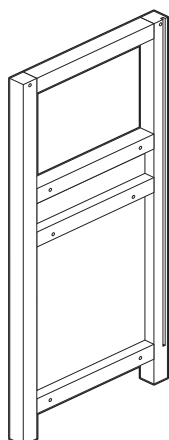
1 Left side x 1 (72.5(h) x 32(d)cm)
