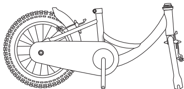
Frame Assembly
