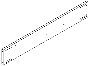
4 Side Rail 4FT: 1925x305 mm 4FT6: 1925x305 mm 5FT: 2010x305 mm
