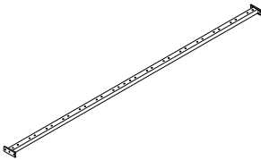
13 Center Rail 4FT: 1828 mm 4FT6: 1828 mm 5FT: 1908 mm
