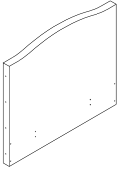
1 Headboard 4FT: 1270x1240mm 4FT6: 1440x1240 mm 5FT: 1590x1240 mm
