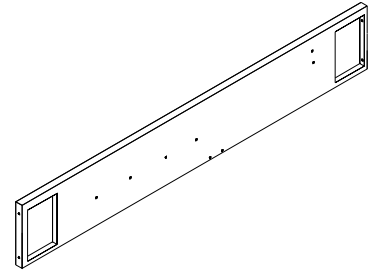
3 Side Rail 4FT: 1925x305 mm 4FT6: 1925x305 mm 5FT: 2010x305 mm
