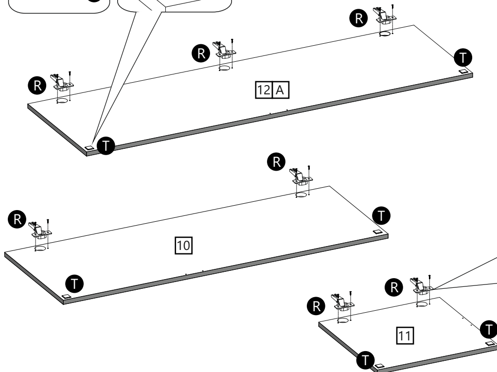
10 Upper Right Door (1231 x 445mm)
