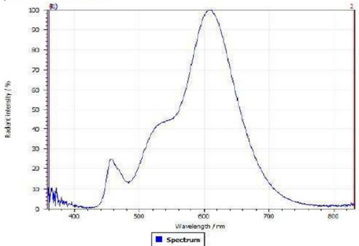
Spectrum of LED module
