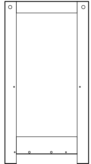
3 Right side panel (70.7 x 36.6cm)
