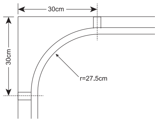
Average right angle bay, approximate bracket position
