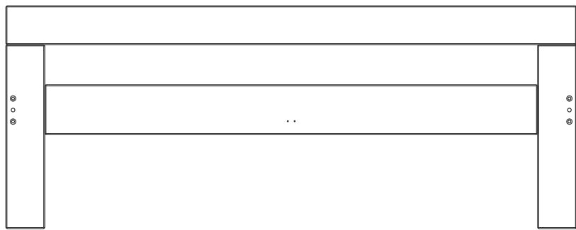
2 Footboard (618 x 1581mm)
