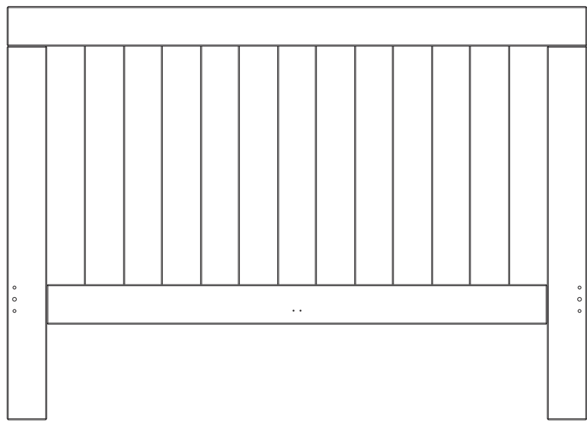
1 Headboard (1128 x 1581mm)
