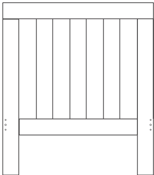
1 Headboard ( 1128 x 971mm )
