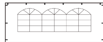
9 Side Panel w/window (x4) (2900 x 1950mm)
