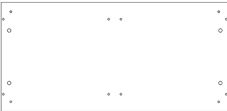
2 Bottom panel x 1 (96x46cm)
