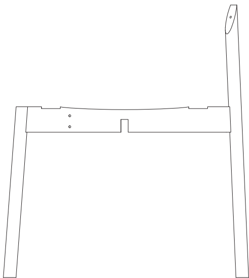
1 Up Leg Frame x 1 (745x 675mm)
