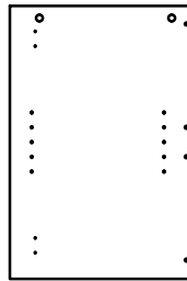
5 Left Side (592 x 391mm)
