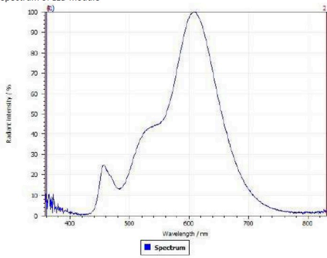
Spectrum of LED module
