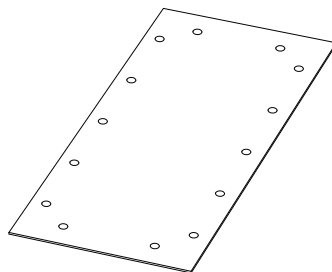
8 Back board x 1 (63.5 x 27.5 x 0.3cm)
