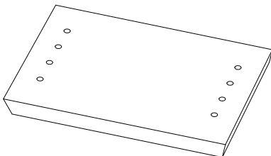
7 Top x 1 (37.5 x 30 x 1.5cm)
