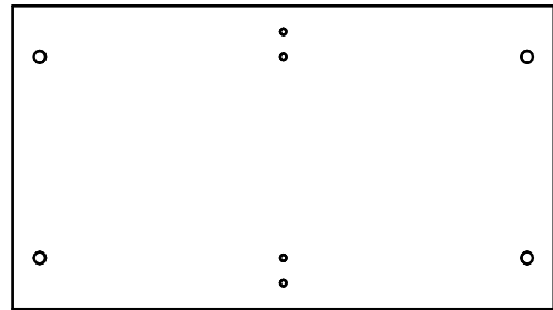
6 Horizontal partition x 1 (69x39cm)
