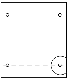
5 Middle vertical partition x 2(34x38cm)
