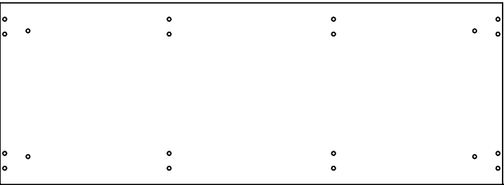
2 Bottom panel x 1(108x39cm)
