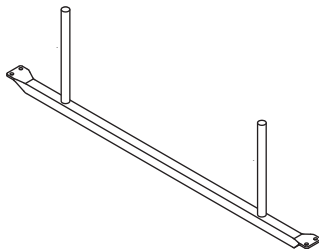
5 METAL RAIL (25x950mm)
