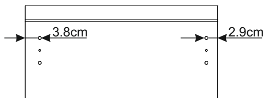
14 Left Drawer front x 1 (50x25cm)
