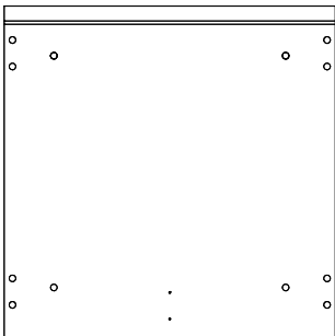
3 Bottom panel x 1 (40x40cm)
