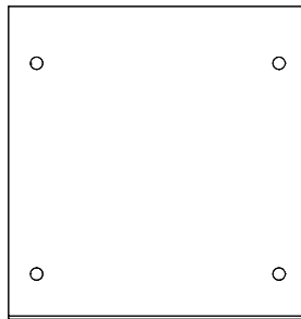
4 Top panel x 1 (36x38cm)
