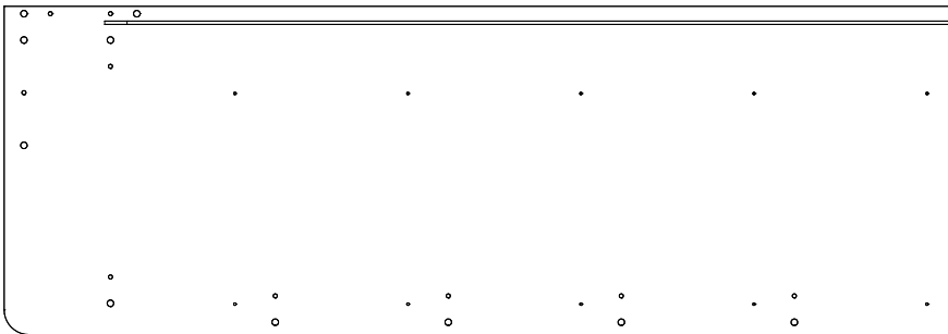
2 Right side x 1 (115x40cm)
