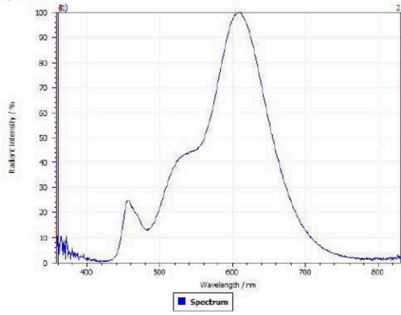
Spectrum of LED module
