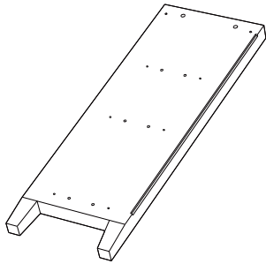
4 Side board on left x 1 (78.2 x 27 x 4cm)
