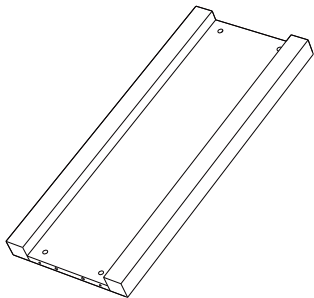
7 Bottom x 1 (63 x 26.5 x 4cm)
