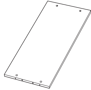
6 Shelf x 2 (63 x 26.5 x 1.5cm)
