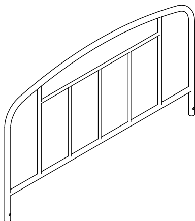
5 Headboard x1 (1248x733mm)
