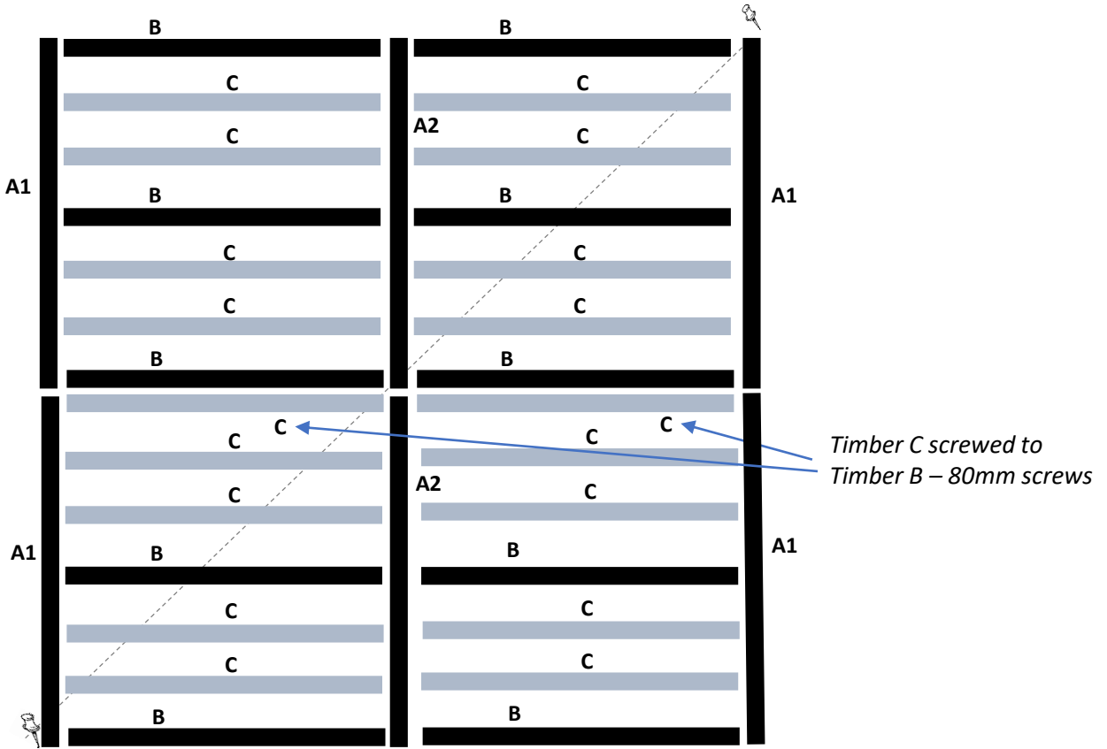
Frame layout — check diagonals are equal
