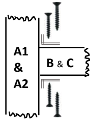
30mm screws through joist hangers
