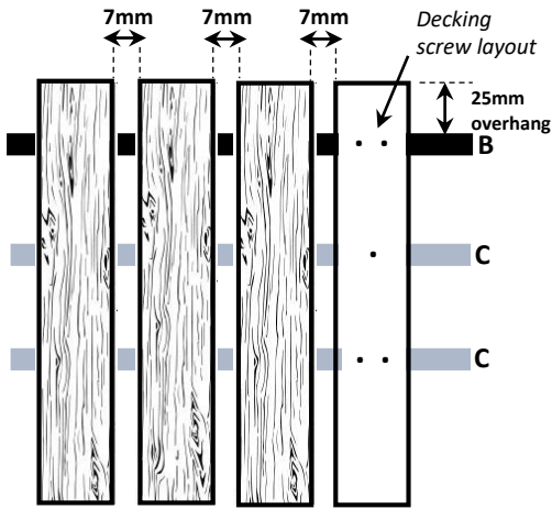
Decking board positions
