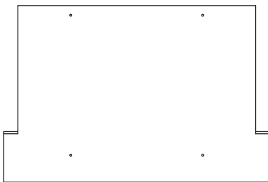
4 Bottom Panel x 1 (385 x 255mm)
