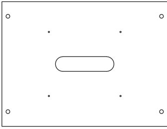
1 Top Panel x 1 (340 x 255mm)
