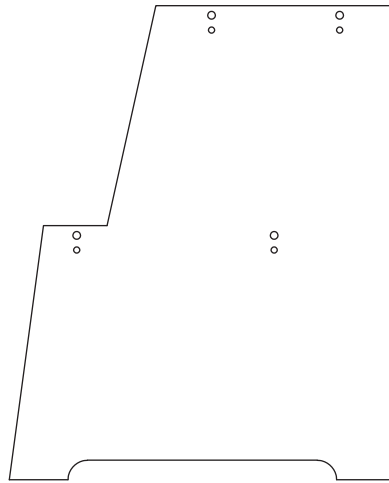
2 Left Side Panel x 1 (490 x 395mm)
