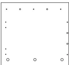
4 Left Side Panel x1 (400 x 372mm)
