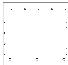
6 Right Side Panel x1 (400 x 372mm)
