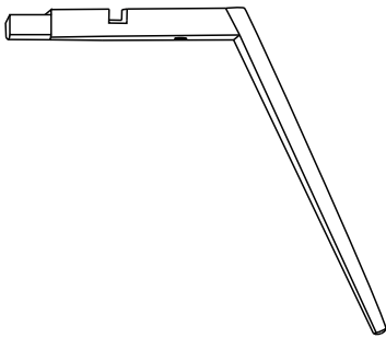
3 Back Leg (Left) x1 (430 x 235 * 20 mm)
