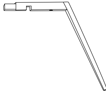
4 Back Leg (Right) x1 (430 x 235 * 20mm)
