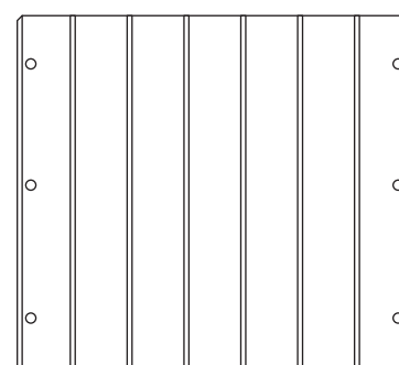
7 Drawer Side x 4 (22x24.5cm)
