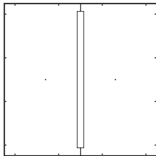
6 Back (69.8 x 69.8cm)
