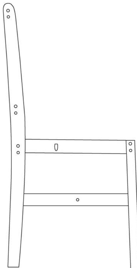
2 Right side frame (41 x 88cm)
