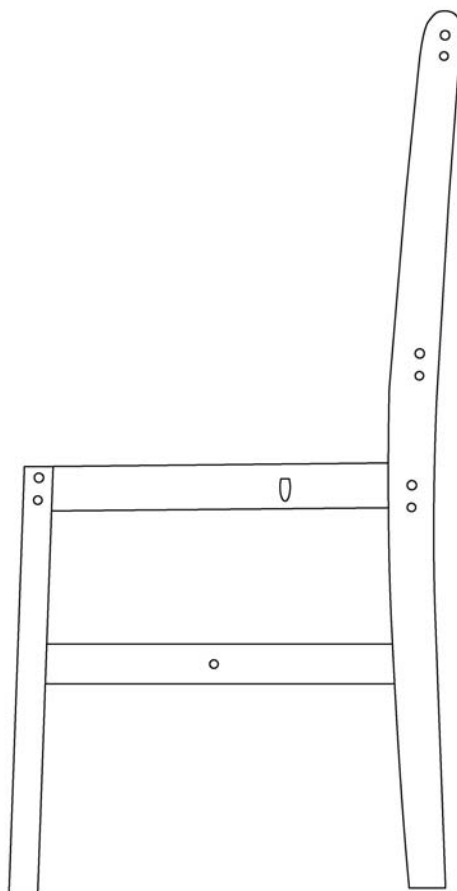
1 Left side frame (41x88cm)
