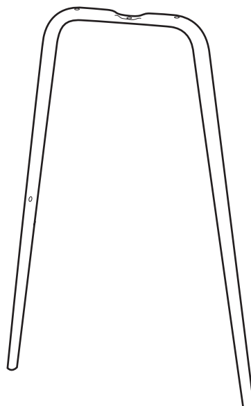
4 Lower leg (Ø2.2 x 72 x 47cm)
