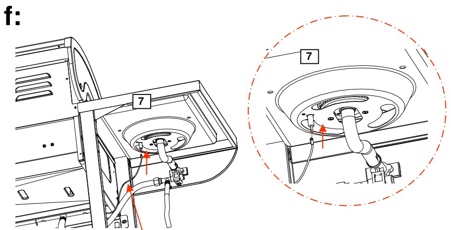
side burner electrode wire
